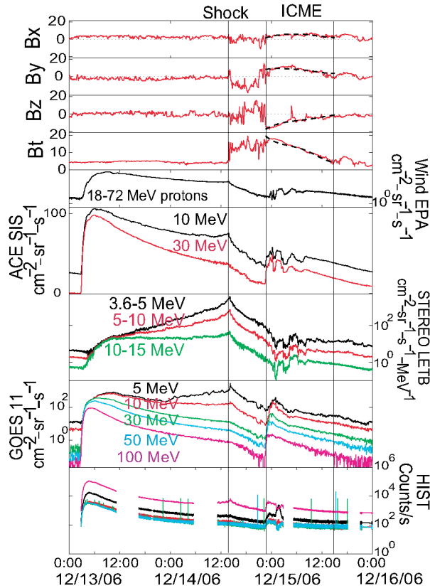
FIGURE 1. Time series plot of ACE magnetic field in GSE coordinates and the December 13 and 14, 2006 SEP events observed at Wind (integral rate), ACE (integral rate), STEREO LET B (differential rate), GOES 11 (integral rate), and Polar HIST (count rate). Note the December 14 SEP event occurs just after a shock and within an ICME (marked by the vertical lines) and exhibits a quasi-oscillatory time profile, especially at lower energies.
