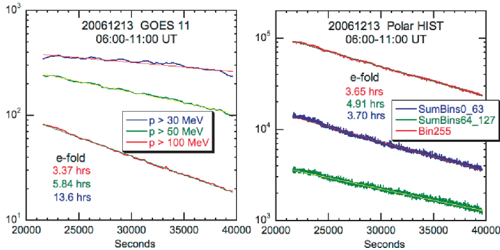
FIGURE 2. Energetic particle intensity decay of the December 13, 2006 SEP event as observed at GOES 11 (left panel) and Polar HIST (right panel). Decay was exponential with a large number of protons \geq 100 MeV. The calibration interval, 0600 UT -1100 UT, is chosen to maximize the decay and minimize the influence of the radiation belts, truncated 1 hr prior to Polar crossing into the belts. HIST data are divided into 4 sums of 64 bins (bin sums [0, 63] and [64,127] are shown). All pulses larger than 10 MeV appear in overflow bin 255. The e-fold time of HIST is 3.65 hrs similar to the GOES 100 MeV channel with e-fold time of 3.37 hrs.
