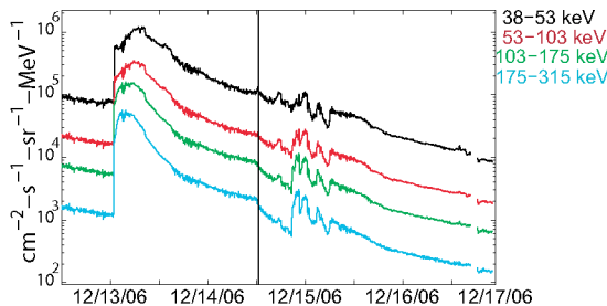
FIGURE 3. ACE EPAM differential electron flux data shown at 38 keV to 315 keV energies. Note the short-scale modulation is clear at all energies.
